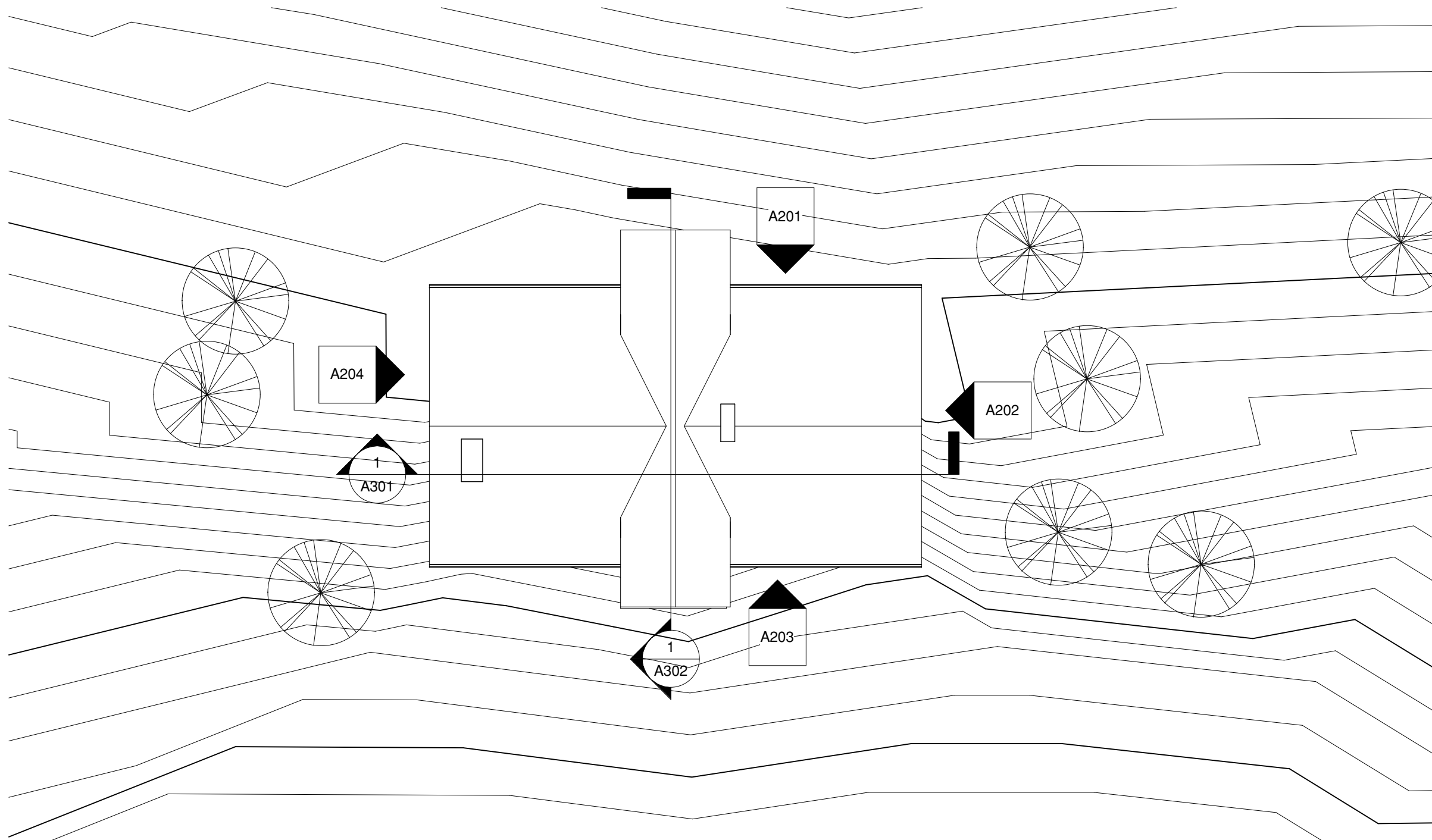
1 Roof View 1/16" = 1'-0"
